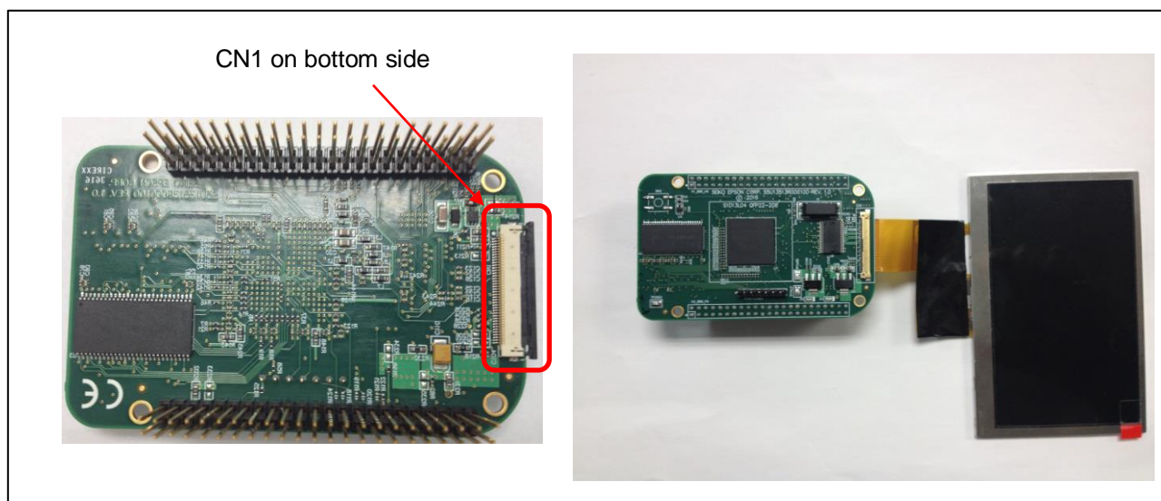
CN1 Location and Panel Connection Example
